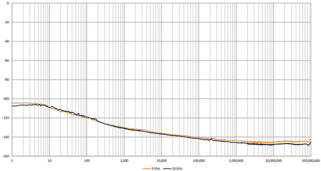
Figure 7. Measured AM noise using the internal LO mode for the N5194A.
